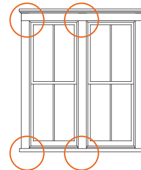
Alternate two-wide double-hung grouping. Jamb and mullion trim widths must match and be approximately 4 1/2" wide for central rosette to fit. Circled areas – See Typical Trim Conditions details on page 13.
