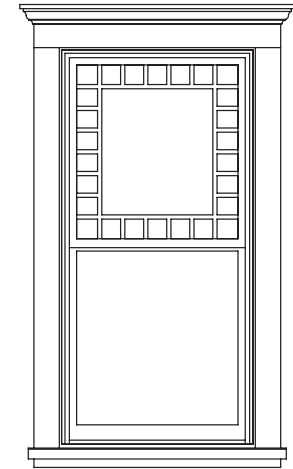
Flat casing for jambs and head with 3 5/8" cornice. Extended sill nose with apron.
