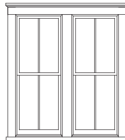
Two-wide double-hung grouping. +/- 5 1/2" mull is a very authentic size.
